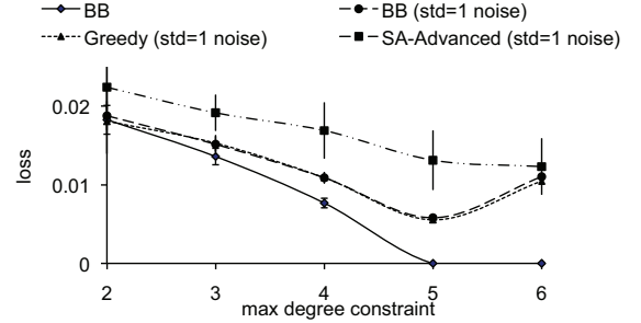
Figure 3: Loss when the entire game is sampled and added noise for tree graph cases
