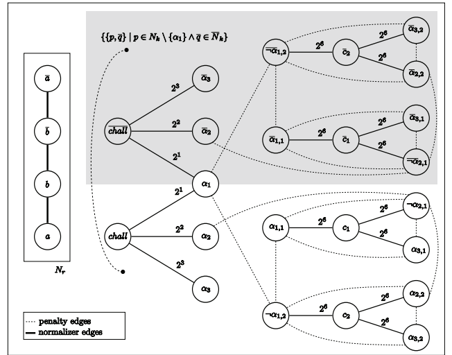
Figure 2: The game N(\hat{\phi}) , where \hat{\phi} = (\alpha_1 \vee \neg\alpha_2 \vee \alpha_3) \wedge (\neg\alpha_1 \vee \alpha_2 \vee \alpha_3) .
