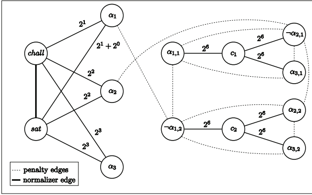
Figure 1: The game K(\hat{\phi}) , where \hat{\phi} = (\alpha_1 \vee \neg\alpha_2 \vee \alpha_3) \wedge (\neg\alpha_1 \vee \alpha_2 \vee \alpha_3) .
