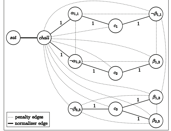
Figure 3: The game BS(\hat{\Phi}) , where \hat{\Phi} = (\forall \alpha_1)(\exists \beta_1, \beta_2, \beta_3)(\alpha_1 \vee \neg \beta_1) \wedge (\neg \alpha_1 \vee \beta_1) \wedge (\beta_1 \vee \beta_2 \vee \neg \beta_3) .
