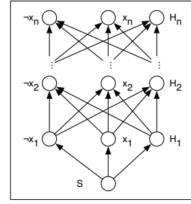
Figure 3: The graph constructed by the seeker BR reduction for a SAT instance with n literals.
