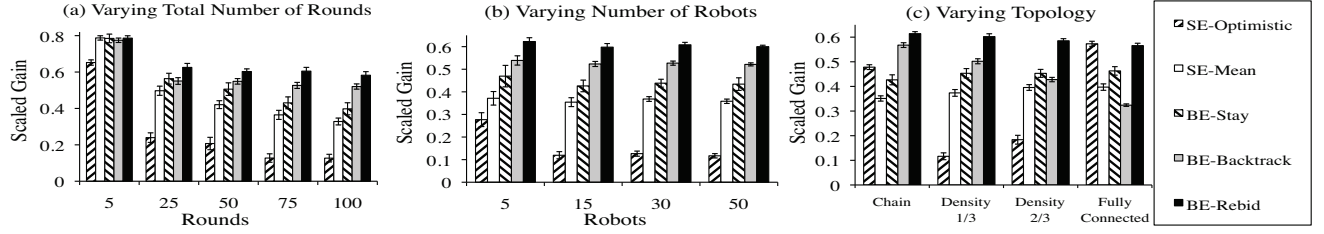
Figure 4: The performance of different algorithms is shown where the y -axis is the scaled gain (0 represents No-Movement and 1 represents the gain of MGM-Omniscient), the x -axis describes the setting, and the error bars show standard error.
