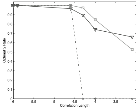
Figure 4: Optimality rate results for 6 agents and 6 issues with different constraint widths.
