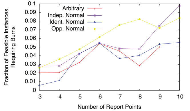
Figure 3: The fraction of feasible instances requiring money to be burnt increases in k .
