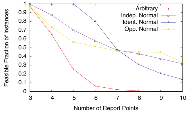
Figure 2: The fraction of feasible instances decreases in k .
