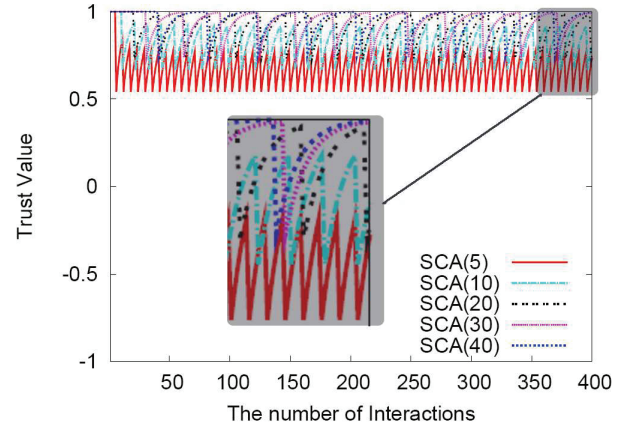
Figure 3: Exploitation of FIRE model by a con-man.
