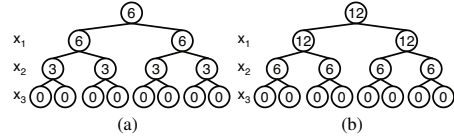
Figure 3: h -Values for the Example
