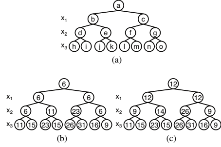
Figure 2: Search Trees for the Example
