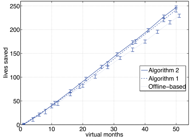
Figure 2: Algorithms 1 and 2, and the offline-based algorithm on generated data. Standard deviations are also shown for each data point. Steady state is from month 26 to month 35.
