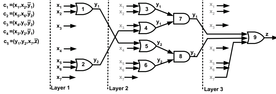
Figure 2 Conversion of a CNF decomposition of a consistency checker into a monotone Boolean circuit.
