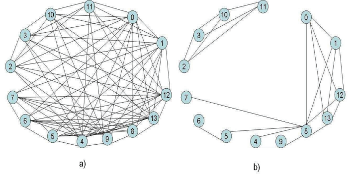
Figure 1: CELAR6-SUB1 Problem
