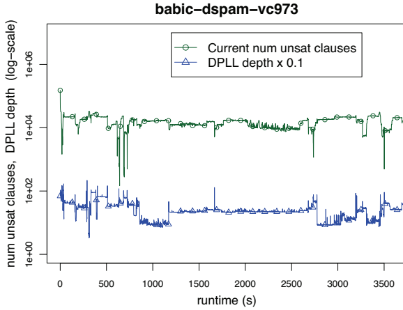
Figure 2: Number of unsatisfied clauses in MiniWalk and DPLL search depth vs. time in babc-dspam-vc973.cnf.
