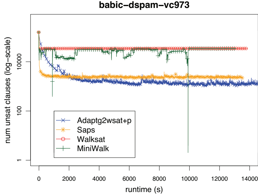
Figure 1: Qualitative search behavior in terms of the number of unsatisfied clauses (y-axis, log scale) as runtime progresses (x-axis). Both state-of-the-art pure local search methods, unguided Walksat and MiniWalk are shown. Note the deep drops of MiniWalk, which distinguish it from the other techniques. Instance: babc-dspam-vc973.cnf.
