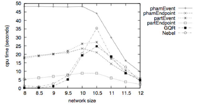
Figure 6: Average CPU time against network degree, for networks of size 50–100; 3000 instance per datapoint.
