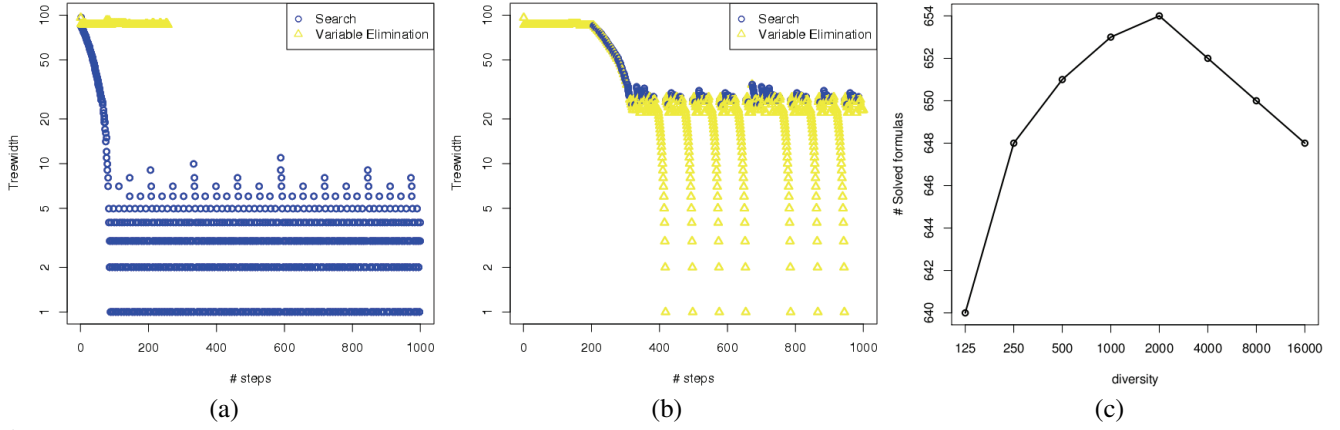
Figure 3: (a) Number of reasoning steps ( x axis) vs. approximated treewidth value ( y axis) in STRUQS[VE] (triangles) and STRUQS[BJ] (dots). (b) As (a), but describing the alternation of search (dots) and variable elimination (triangles) steps inside STRUQS[BJ,VE]. The number of reasoning steps corresponds to the number of LS- and VE-type records pushed on \Gamma . In particular, we consider the sequence of QBFs \varphi_1, \varphi_2, \dots where \varphi_1 is the input QBF, and \varphi_{i+1} is obtained from \varphi_i as follows. If \varphi_i does not correspond to a conflict or a solution, then \varphi_{i+1} is the result of a destructive update of \varphi_i corresponding to (i) unit propagation and (ii) variable elimination or search. If \varphi_i is a conflict or a solution, then \varphi_{i+1} is the formula corresponding to the node where STRUQS backtracks to. For all \varphi_1, \varphi_2, \dots , approximated treewidth \hat{tw}_p(\varphi_i) is such that tw_p(\varphi_i) \leq \hat{tw}_p(\varphi_i) . (c) Number of formulas solved ( y axis) vs. div parameter value ( x axis) in STRUQS[BJ,VE].
