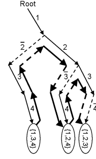
Figure 4: Depth-first search in a binary decision tree can be used to order node expansions in breadth-first treewidth computation.
