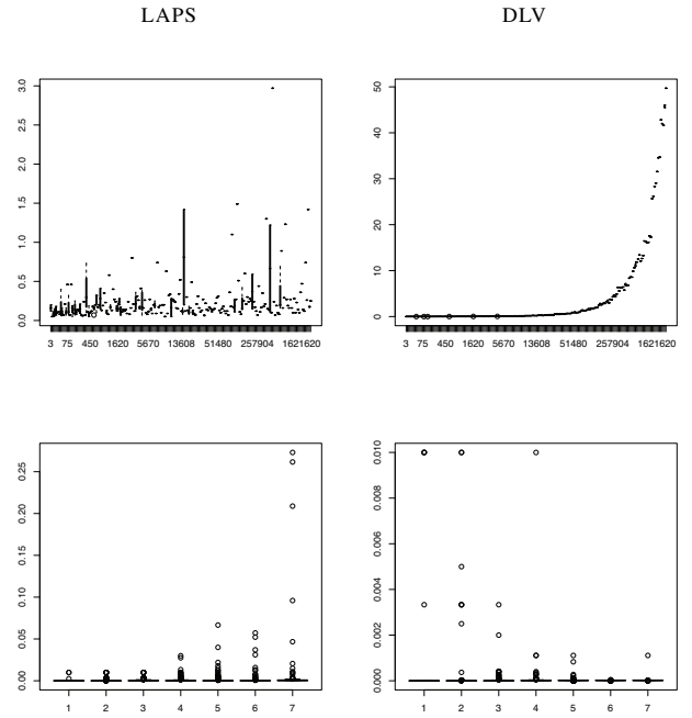
Figure 5: Comparison of the runtime behavior.
