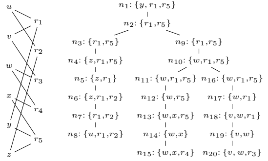
Figure 1: Incidence graph G_P of example program P (left) and a normalized tree decomposition T of G_P .
