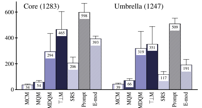
Figure 2: Module sizes for |\Sigma| = 10 and standard deviation.
