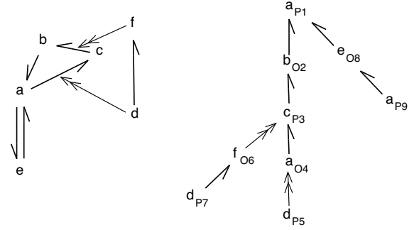
Figure 3: An EAFs and \phi_{PC} winning strategy for a
