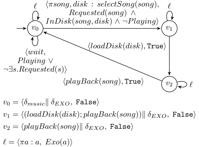
Figure 1: Characteristic graph for program \delta_{\text{music}} .
