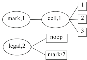
Figure 2: A dependency graph for calculating domains of functions and predicates. (Ellipses denote argument positions of functions or predicates, and rectangles denote function symbols themselves, including constants.)
