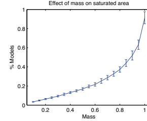
Figure 7: Surprisingly, the effect of mass on the final fraction of domain-specific models is approximately quadratic, rather than linear as might have been anticipated.
