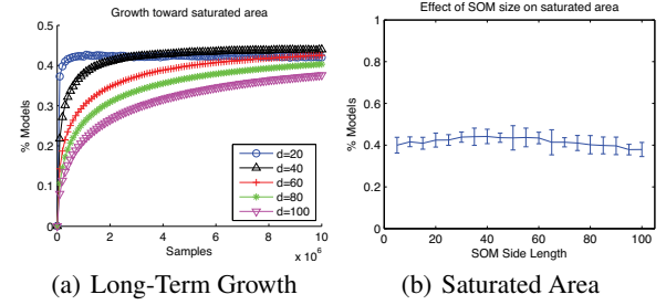
Figure 6: Once the spike begins to occupy a significant fraction of the SOM’s model, it converges exponentially towards a final equilibrium. Larger SOMs converge more slowly (a) but all sizes arrive at approximately the same equilibrium (b).
