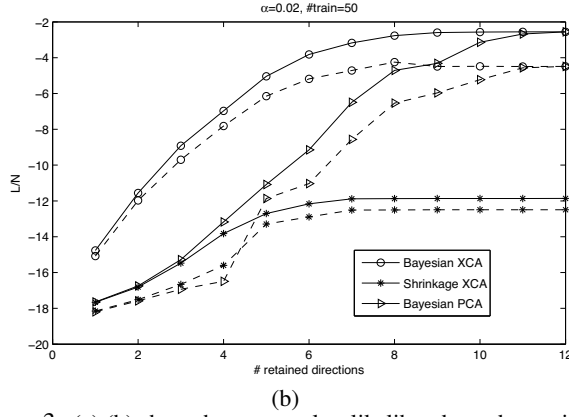
Figure 3: (a),(b) show the average log-likelihood per data point of the Mosquito Wing Landmark data on the training set of 50 data points (solid) and test set of 77 data points (dashed) as a function of the number of retained directions. (a) compares Bayesian XCA with XCA and PCA, and (b) compares Bayesian XCA with Bayesian PCA and Shrinkage XCA. Hyper-parameter \alpha = 0.02 is determined through cross validation with d = 5 . The inset shows the number of minor components for different numbers of retained directions for Bayesian XCA (o) and XCA (x).
