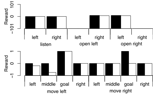
Figure 2: Result of IRL from FSC policies. Top : Tiger problem. Bottom : 1d maze problem. Black bars : The true reward. White bars : The estimated reward.
