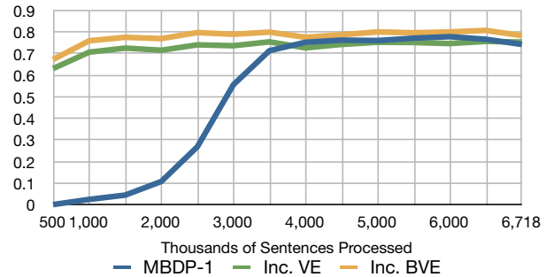
Figure 6: Results of comparison in the incremental paradigm. Each point represents the performance (boundary-based F-score) of that algorithm on the previous 500 sentences.
