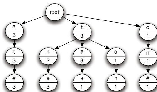
Figure 2: A portion of the knowledge trie built from #the#cat#sat#on#the#mat#. Numbers within each node are frequency counts.
