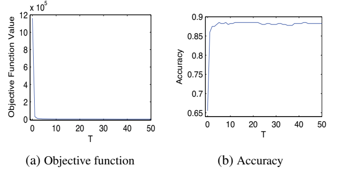
Figure 2: Convergence properties of RRMF.
