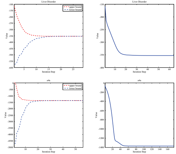
Figure 1: Convergence plots. Figures in the first column correspond to the level method, and figures in the second column correspond to the constrained gradient descent method.
