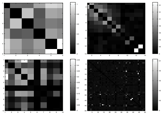
Figure 2: The different dependency structures discovered by LMBMr for different datasets. The colorbar of each figure shows the scale of weights in terms of the gray level (absolute value). The top row, left to right: Scene and Yeast ; The bottom row, left to right: Mediamill10 and Mediamill50 .
