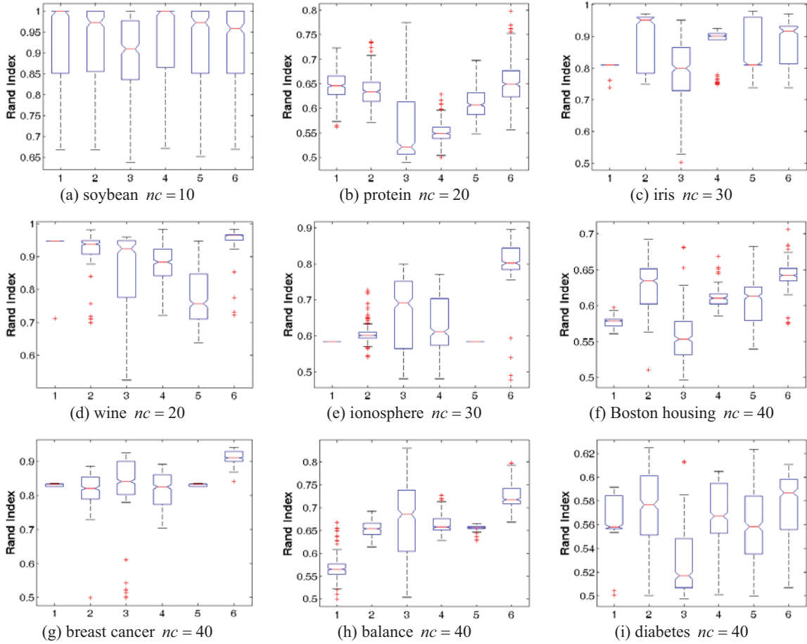
Figure 3. Clustering results on the nine UCI data sets using different metrics (numbered as in Section 3.1).
