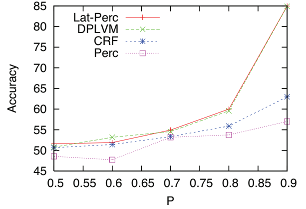
Figure 3: The curves of the latent perceptron (Lat-Perc), DPLVMs, perceptron (Perc) and CRFs, when P varies.
