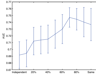
Figure 2: Performance on Ligand
