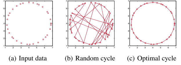
Figure 1: Finding the most ordered cycle through entropy minimization. (a): the input data sampled from a circle; (b): a random order with a higher entropy; (c): the optimal cycle with the minimal entropy 0.384314.
