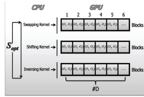
Figure 4: The block-level design of FATS. Each kind of kernel is implemented as a separate call to GPU. There are totally \#D blocks of each kernel. The entropy S_{opt} is updated alternatively in the loop.
