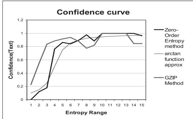
Figure 6: The graph shows the curve obtained by plotting confidence value for classification of TEXT for the strokes in the training data against their entropy values. On the zero-order entropy curve (dark bold line), the entropy value 3.55 corresponds to a confidence value of 0.5; in other words, equal numbers of text and shape strokes had an entropy = 3.55 in the training data. The bold gray line shows the same plot when GZIP entropy was used. GZIP entropy values have been scaled for comparison.
