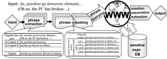
Figure 2: Flow chart of the Web mining technique.
