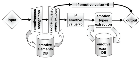
Figure 1: Flow chart of the ML-Ask system.
