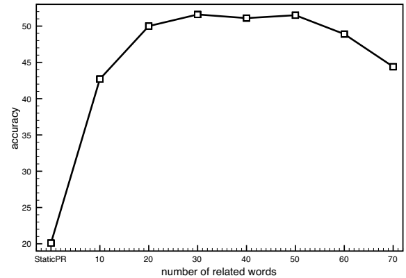
Figure 1: Learning curves for PPR (Sports) using different numbers of related words from the distributional thesaurus. Leftmost point is null context, which equals to static PR.
