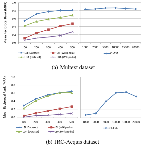
Figure 1: Results for the mate retrieval experiments on English and French documents for different topic numbers for LSI/LDA and different ESA vector lengths for CL-ESA.
