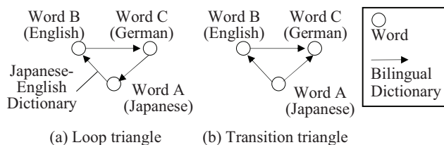
Figure 3. Two types of shapes of triangles
