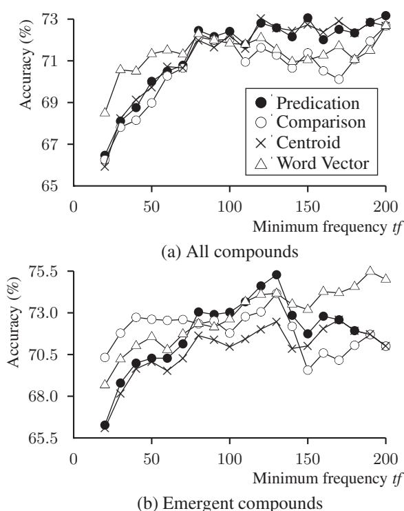
Figure 1: Accuracy of MCS tests as a function of minimum frequency of compounds
