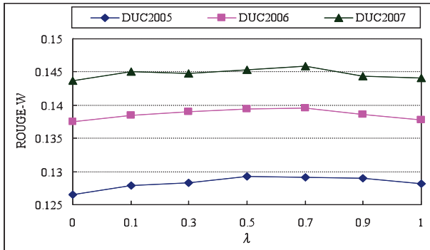
Figure 4: ROUGE-W F-measure scores vs. \lambda for "MultiMR(COM)"
