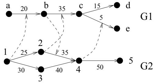
Figure 2: A SAS+ task with two DTGs. Action costs are shown on edges. All edges are distinct actions, except that (b, c) and (2, 4) are the same action. The dashed arrows show precondition of actions.
