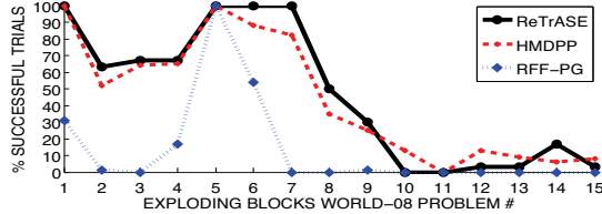
Figure 7: RETRASE outmatches all competitors on Exploding Blocks World-08, although by a narrow margin.
