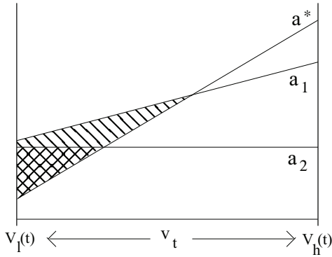
Figure 1: A graphical representation of the VPI_s(t) calculation. Note that a^* is the current greedy optimal action. Gain_{s,t,a^*}(v_t^*) is non-zero for a_1 in the union of the hatched and crosshatched areas and non-zero for a_2 in the crosshatched area. Thus, the action yielding maximal gain is a_1 and the VPI_{s,a^*}(t) is then the combined hatched and crosshatched area multiplied by 1/(V_h(t) - V_l(t)) .
