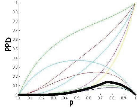
Figure 3: An illustration of proof of Theorem 3, in which the v -neighborhood and v -minimal coincide (here d = 9, t = 5 and v = 3 ). The bold line represents the average of v -neighborhood / v -minimal segments.
