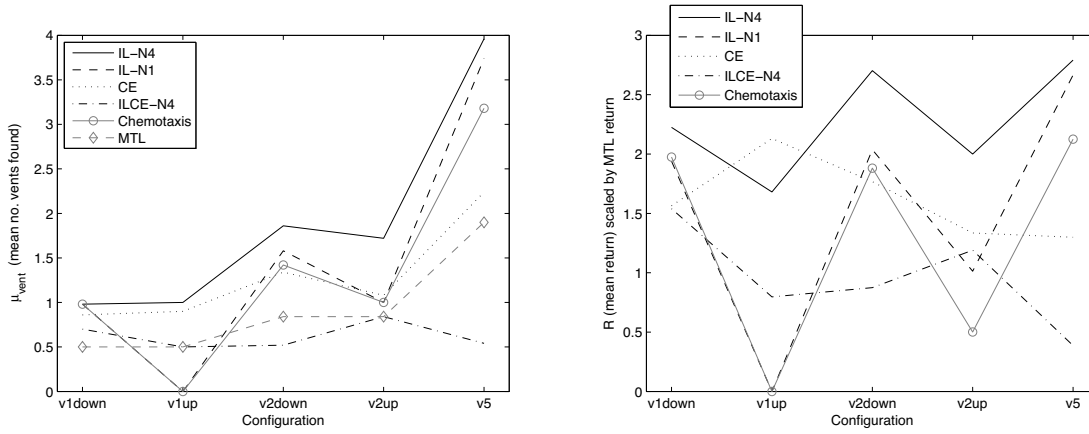
(a) \mu_{vent} , the mean number of vents found. Note the lines connecting data points are purely to aid visualisation.
