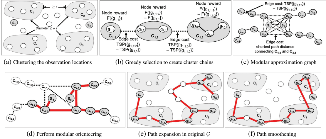
Figure 1: Illustration of nonadaptive informative path planning using PSPIEL OR ( pSPIEL-Orienteering ) algorithm.
