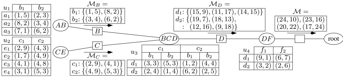
Figure 2: Computing the Pareto set using a GAI network
