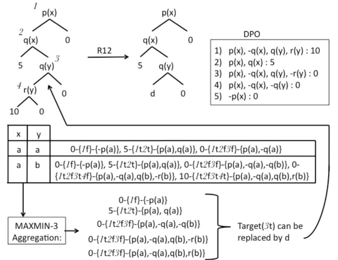
Figure 4: Example of R12 for \max^* \min^* aggregation
