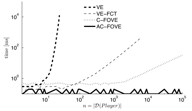
Figure 3: Performance on the model with noisy-OR aggregation.
