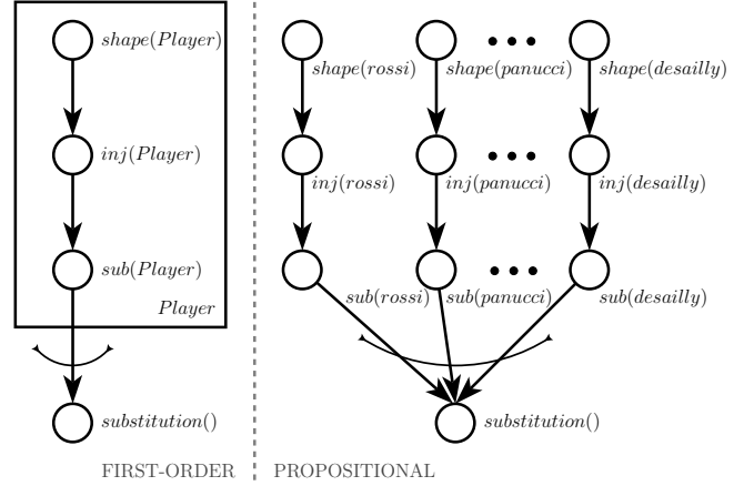
Figure 1: A first-order model from Example 1 and its equivalent belief network. Aggregation is denoted by curved arcs.
