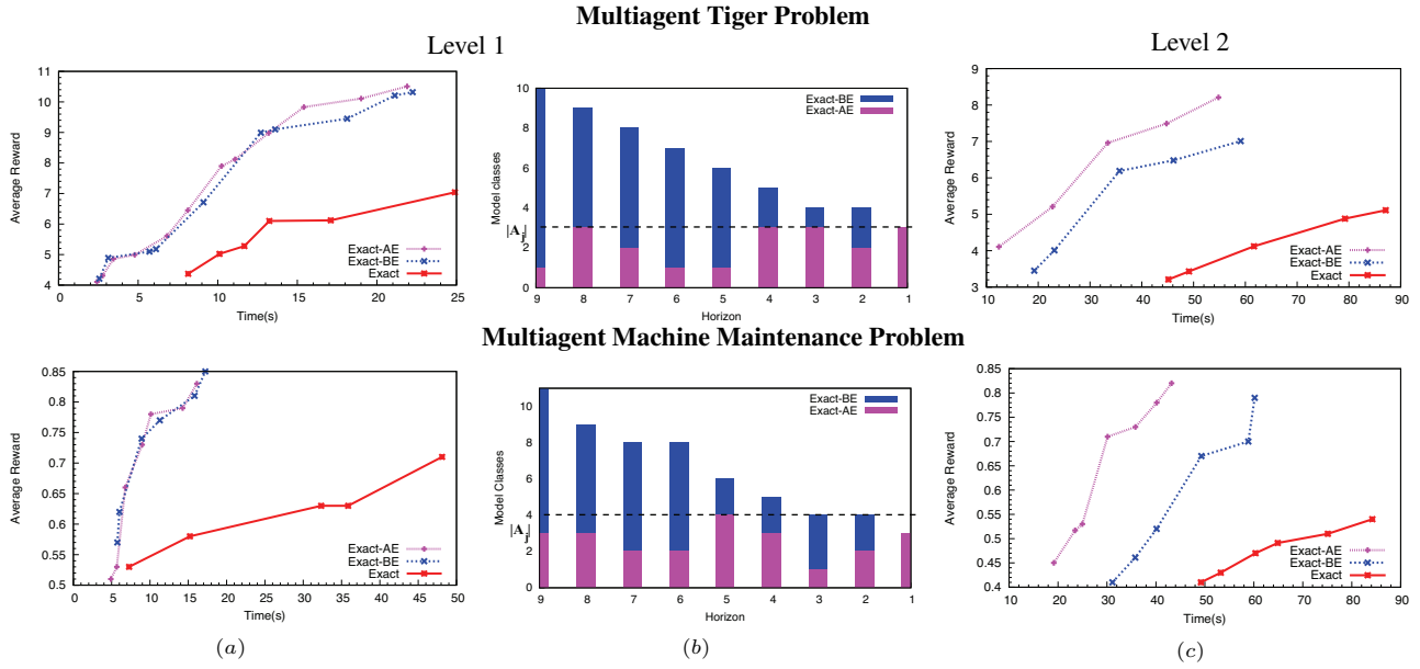
Figure 6: Performance profiles for the multiagent tiger and MM problems generated by executing the solutions obtained using different exact approaches. (a,b) Profiles for level 1 I-DIDs. Notice that Exact-AE maintains less classes at larger horizons in comparison to Exact-BE and never more than |A_j| . (c) Solving level 2 I-DIDs reveals the efficiency facilitated by aggregation using action equivalence.
