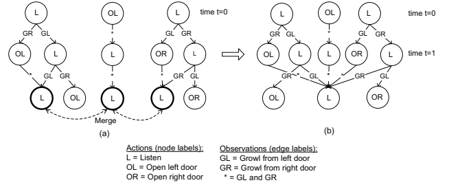
Figure 4: (a) Example policy trees obtained by solving three models of j for the tiger problem. We may merge the three L nodes to obtain the policy graph in (b). Because no policy trees of two steps are identical, no more merging is possible.
