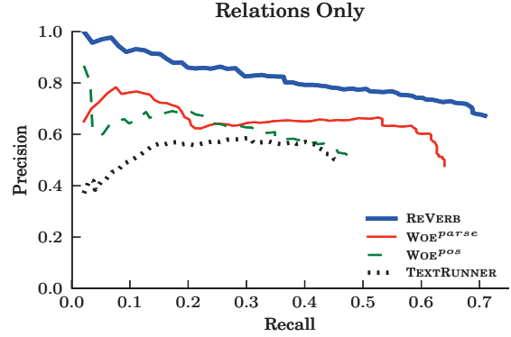
Figure 2: REVERB identifies correct relation phrases with substantially higher precision and recall than state-of-the-art open extractors, including WOEP parse that uses patterns learned over dependency parse paths.
