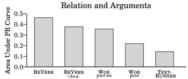
Figure 3: REVERB has AUC more than twice that of TEXTRUNNER or WOEP pos , and 30% higher than WOEP parse for extracting both relation and arguments.
