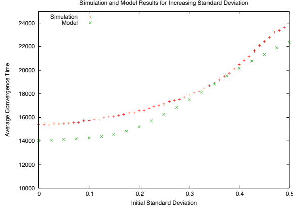
Figure 5: Effects of Initial Standard Deviation on Average Convergence Time, Proportional Update Rule.
